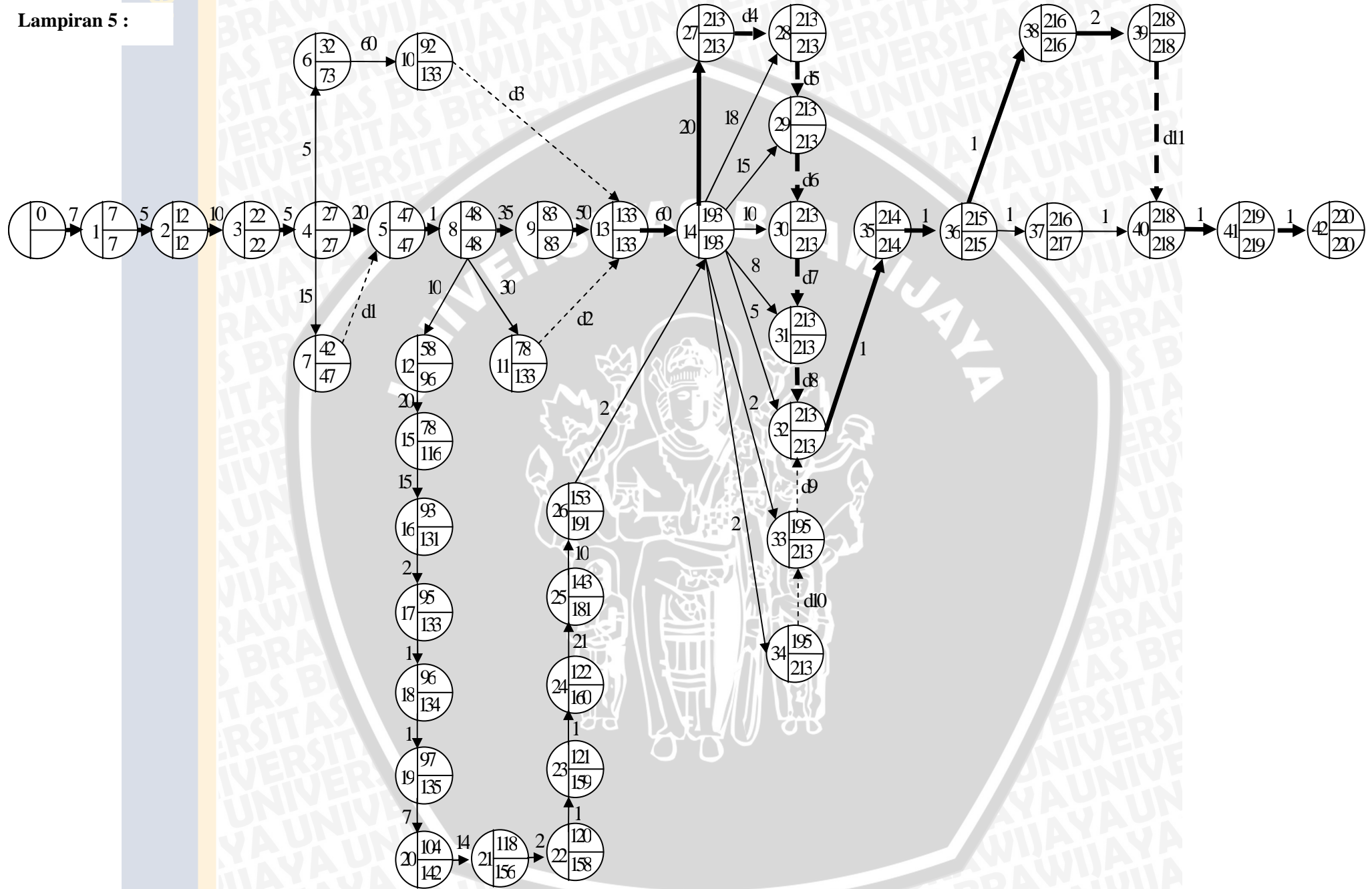
Gambar 4.2 Diagram Lintasan Kritis
