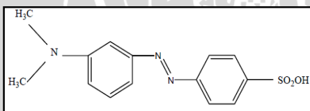
Gambar 2.5 Struktur Methyl Orange (Christina dkk., 2007)
