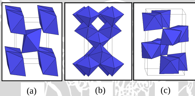
Gambar 2.1 Struktur Kristal \text{TiO}_2 : (a) Rutil, (b) Anatase, (c) Brookite
