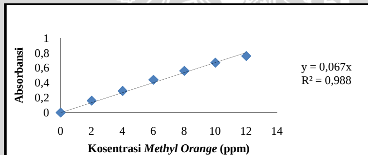
Gambar L.3.2 Kurva Baku Larutan Methyl Orange
