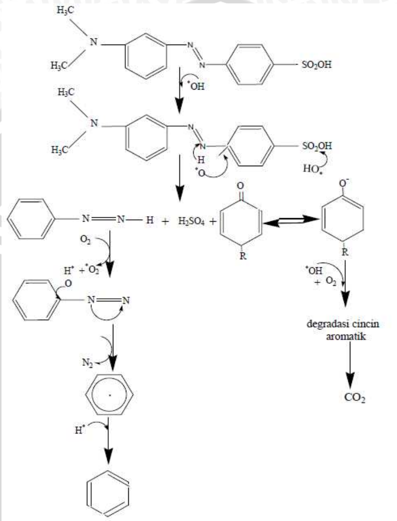
Gambar 2.7 Reaksi Degradasi Methyl Orange (Getoff, 1996)
