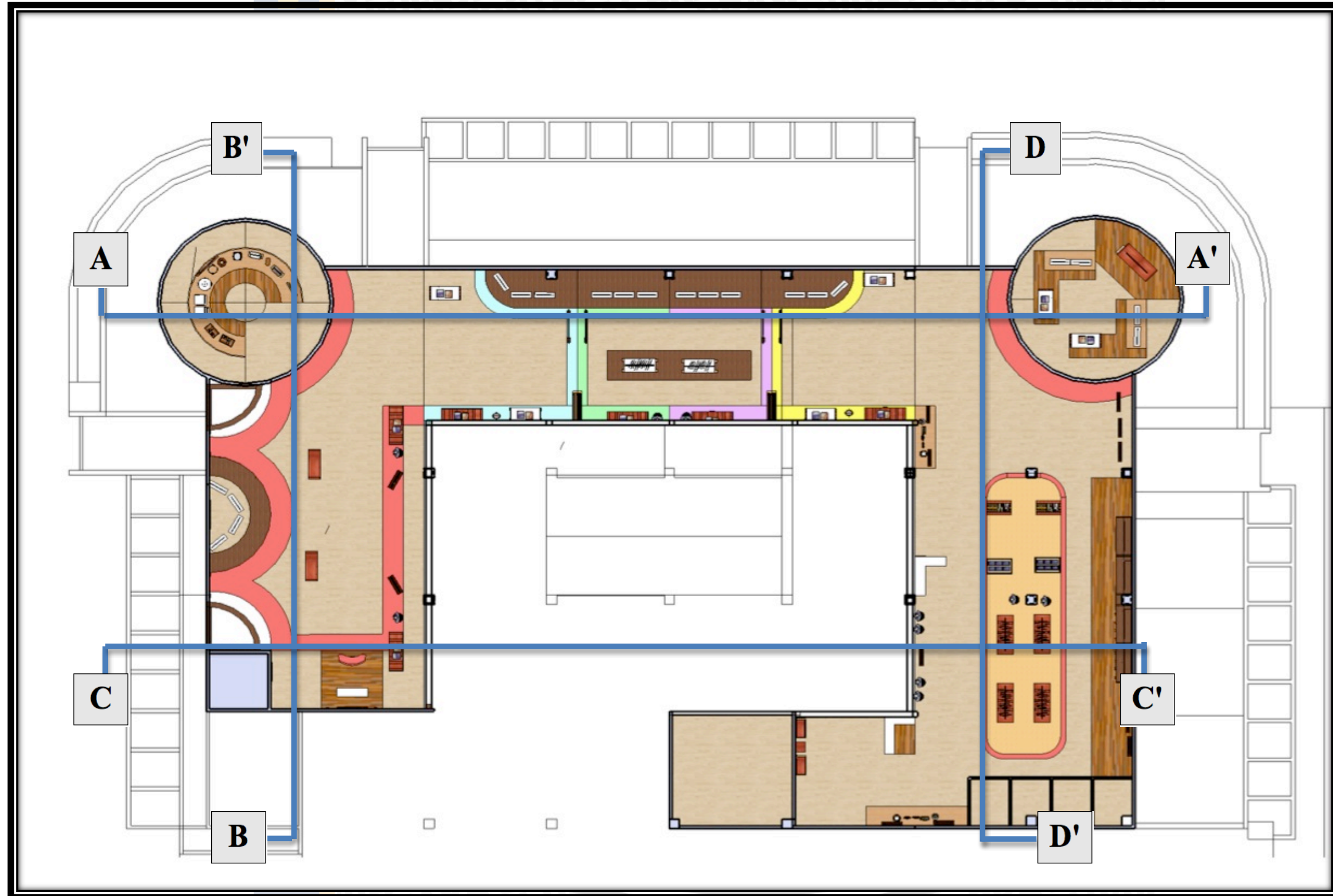
Gambar 4.53 Denah potongan
