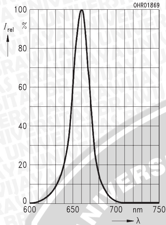
Figure 1. Relative Spectral Emission I_{rel} = f(\lambda)
