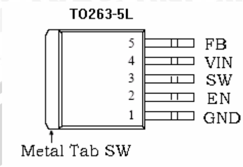
Figure2. Pin Configuration of XL6009 (Top View)
