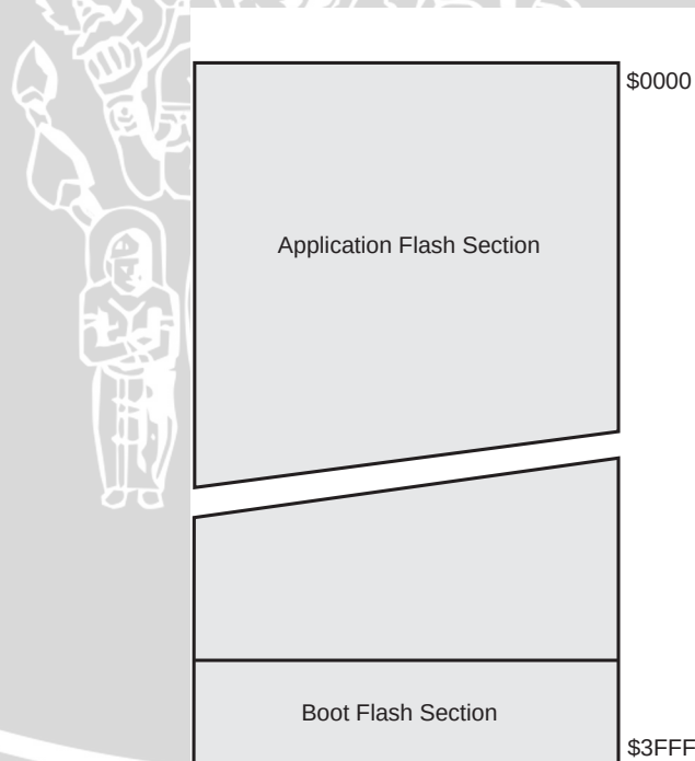
Figure 8. Program Memory Map
