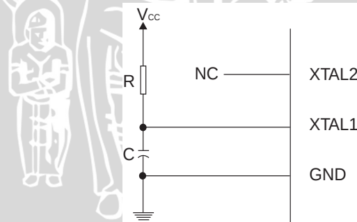
Figure 13. External RC Configuration
