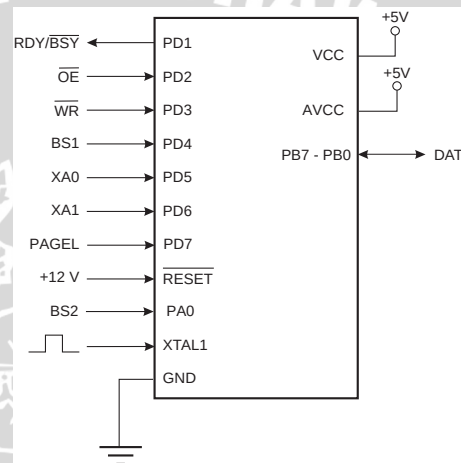
Figure 127. Parallel Programming
