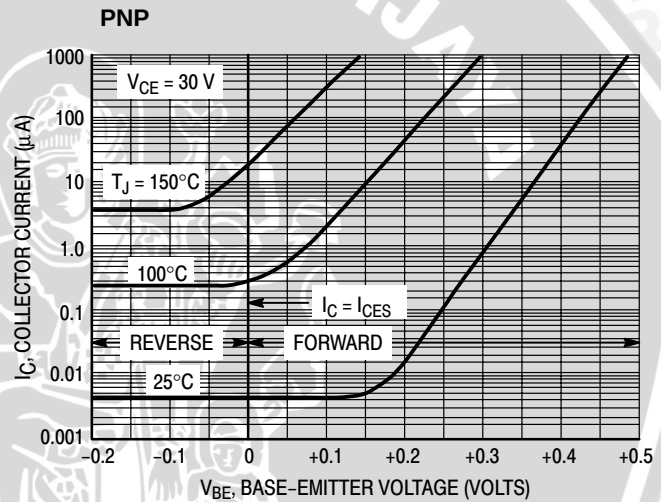
Figure 11. MJ2955A, MJ15016
