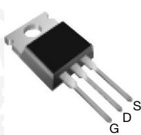
TO-220AB
