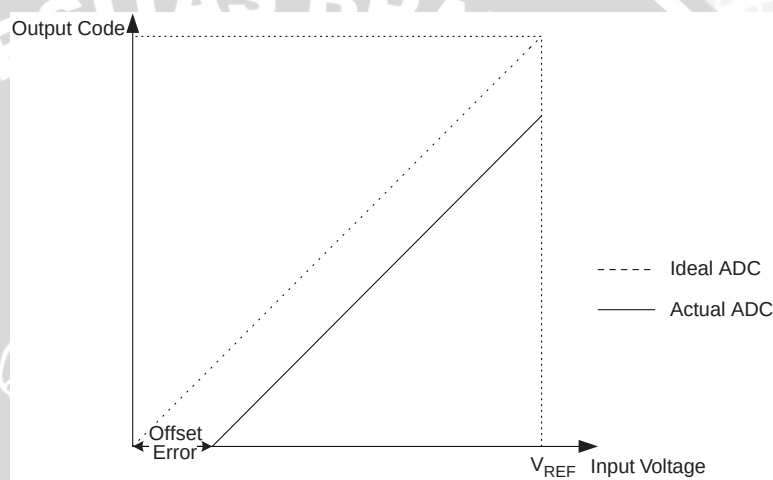
Figure 107. Offset Error
