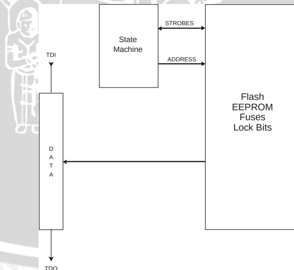
Figure 143. Virtual Flash Page Read Register
