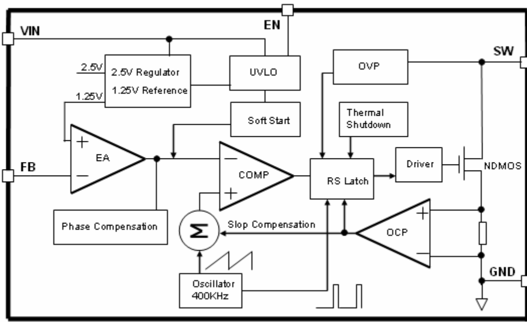
Figure3. Function Block Diagram of XL6009
