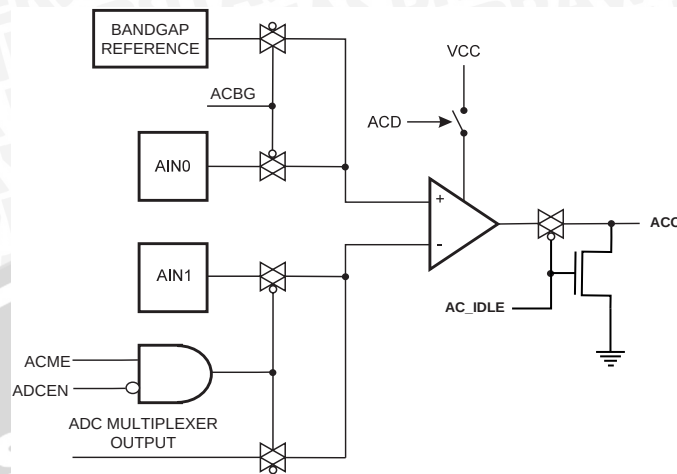
Figure 121. Analog Comparator
