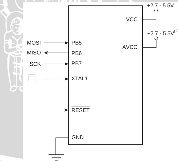
Figure 136. SPI Serial Programming and Verify (1)
