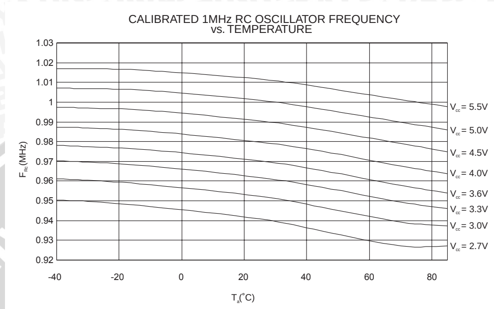
Figure 148. RC Oscillator Frequency vs. Temperature (the devices are calibrated to 1 MHz at V_{CC} = 5V , T = 25^{\circ}C )
