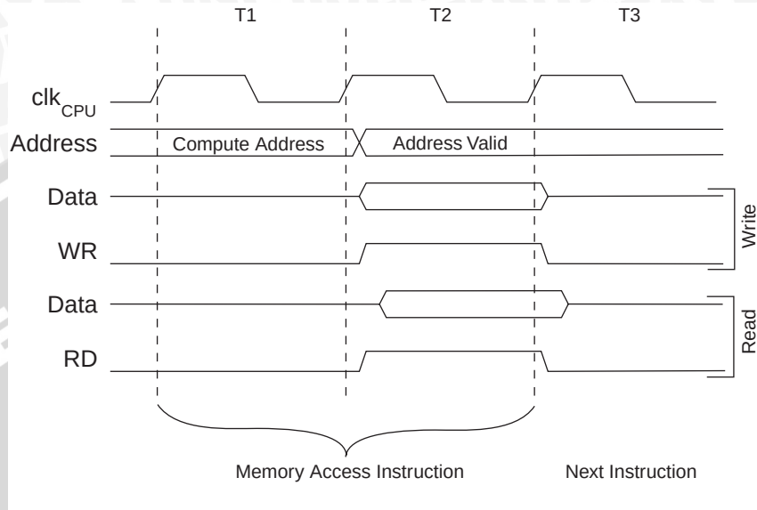
Figure 10. On-chip Data SRAM Access Cycles
