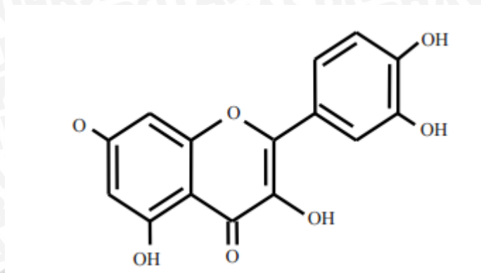
Gambar 2 . Kerangka C_6C_3C_6 Flavonoid (Cuppett et al.,1954)
