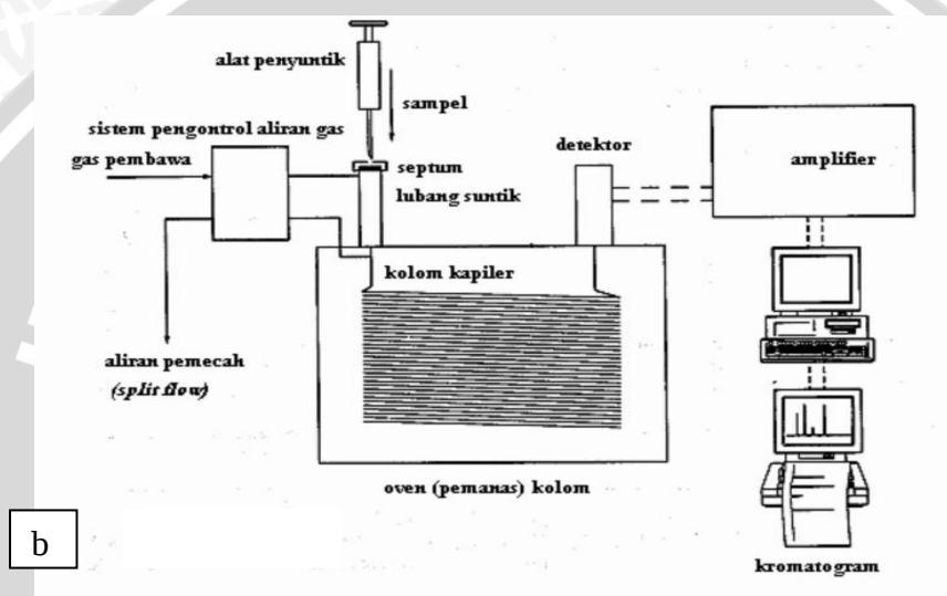
Gambar 6. Gas Chromatography- Mass Spectrometry, (a) alat, (b) Prinsip kerja
