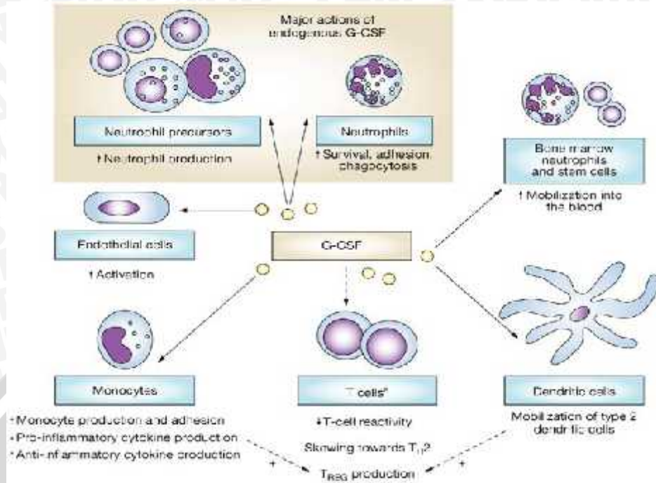
Gambar 2.3 Skema fungsi Granulocyte Colony Stimulating Factor (G-CSF)
