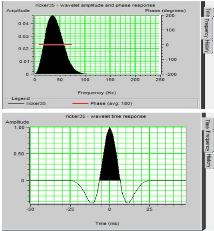
Lampiran 6 Wavelet Ricker 35
