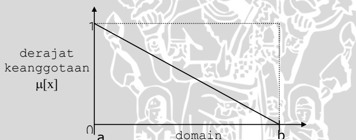
Gambar 7.7 Representasi Linear Turun.
