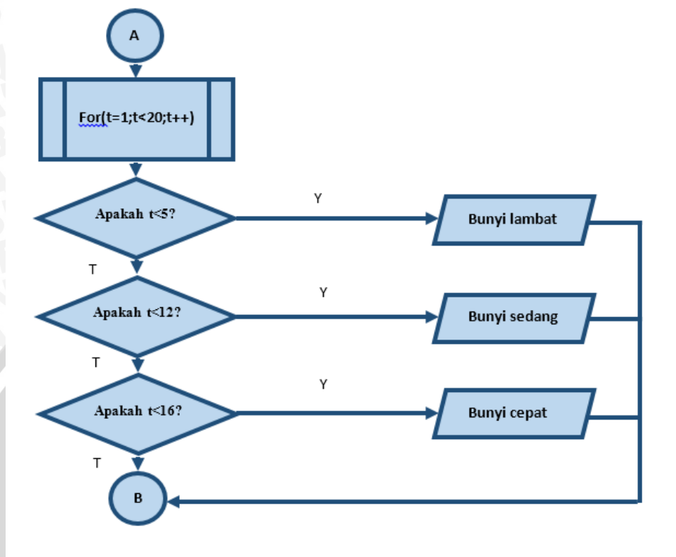
Gambar 5.9 Flowchart Main Program
