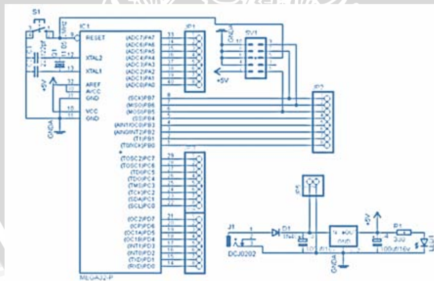
Gambar 4.15 Rangkaian Minimum System
