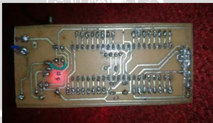
Gambar 5.2b Board Minimum System Tampak Belakang
