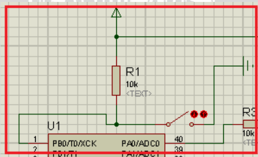
Gambar 4.12 Rangkaian Sensor Adjustabel Infrared
