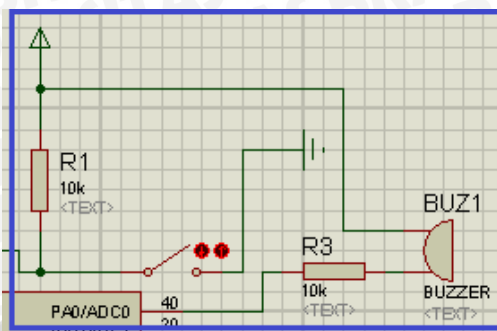
Gambar 4.13 Rangkaian Buzzer
