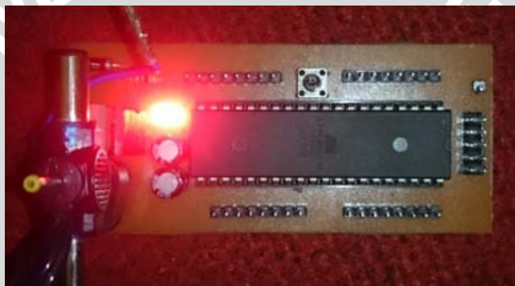
Gambar 5.2a Board Minimum System Tampak Depan
