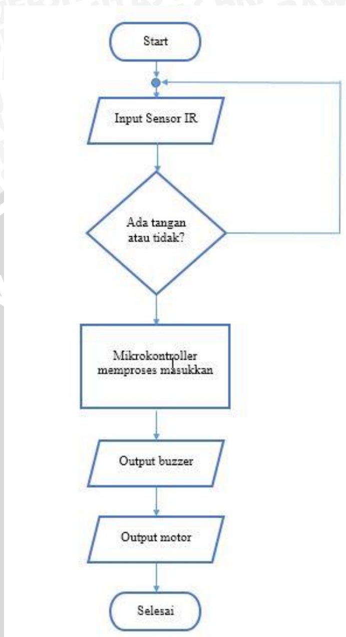
Gambar 4.18 Flowchart Sistem
