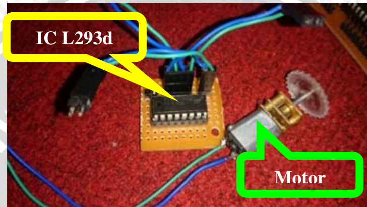
Gambar 5.3 Implementasi Rangkaian Driver Motor
