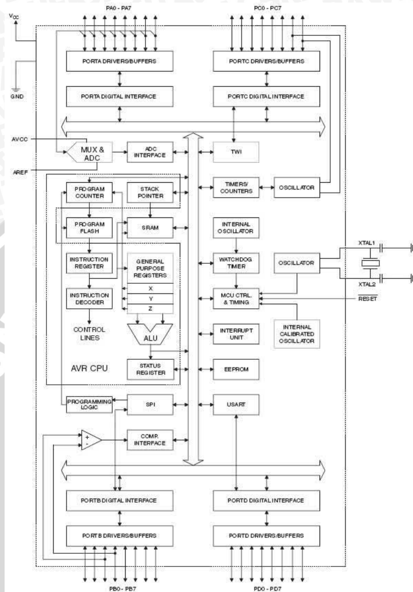
Gambar 2.5 Diagram Blok Mikrokontroler AT8535
