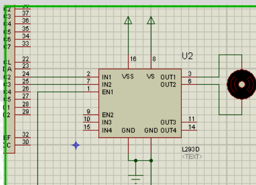
Gambar 4.14 Rangkaian Driver Motor
