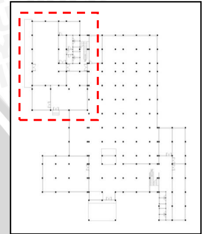
Keyplan Denah Lantai 1
