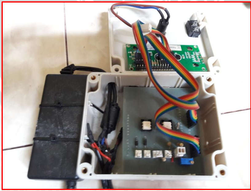
BOX ELECTRIC
