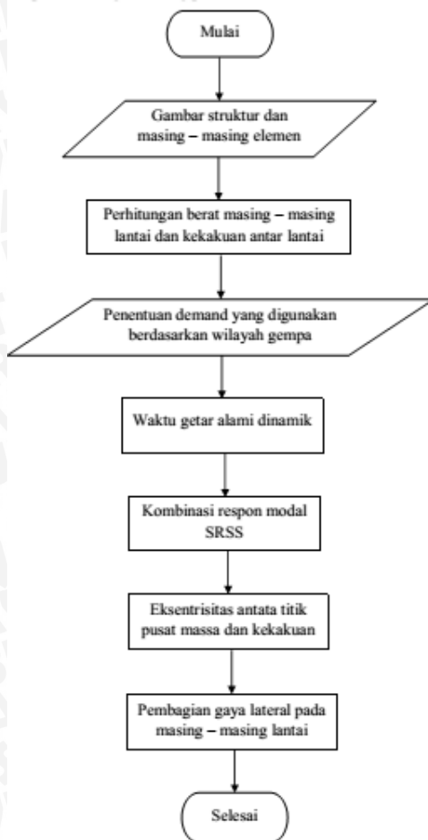
Gambar 6. Flowchart gaya lateral tiap portal.
