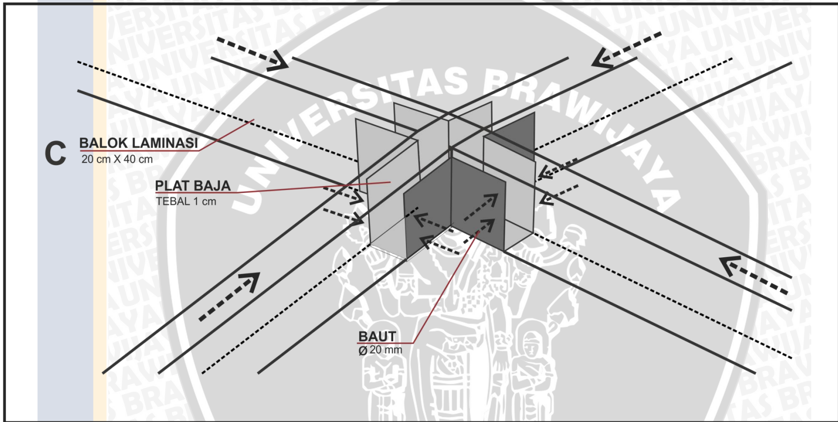
Lampiran 32 Detail Sambungan C Rest Area
