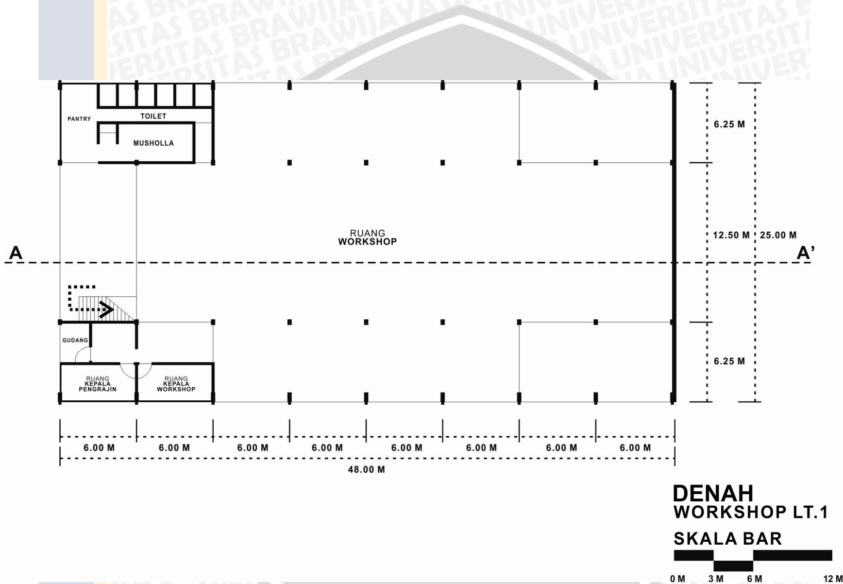
Lampiran 40 Denah Lt.1 Bangunan Workshop
