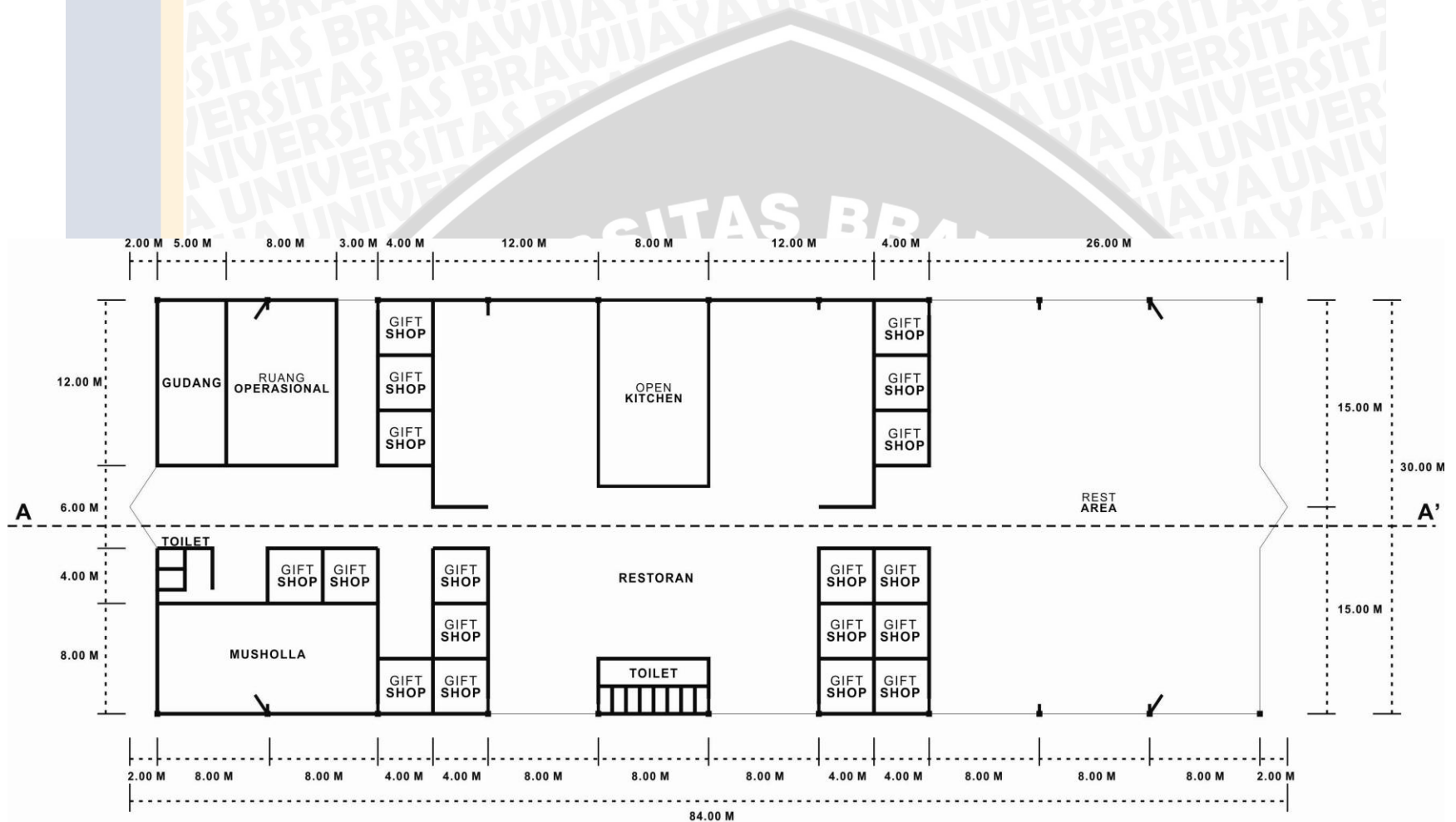
DENAH REST AREA SKALA BAR
