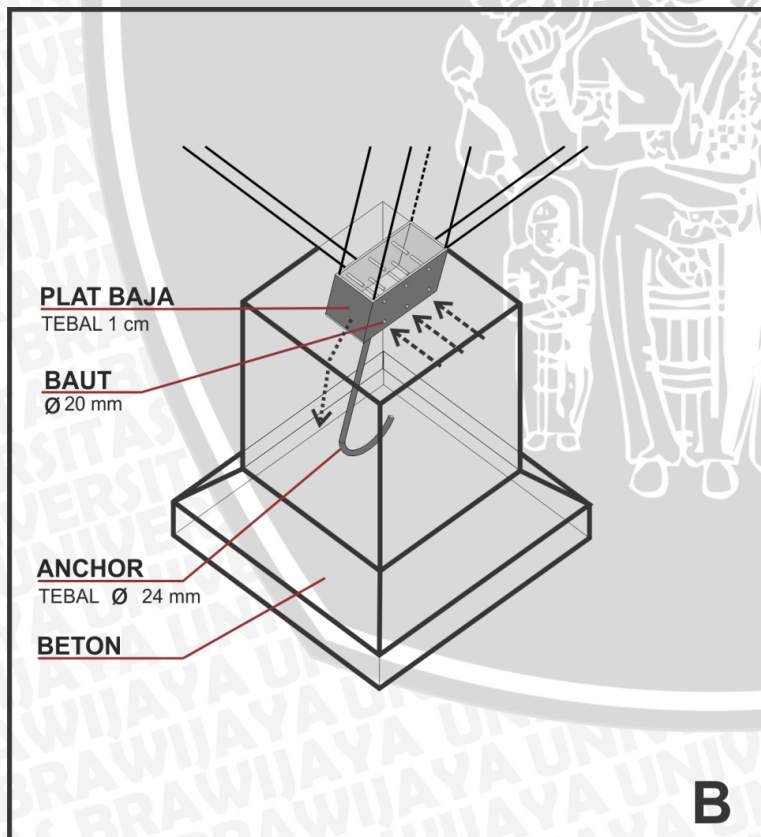
Lampiran 31 Detail Sambungan B Rest Area
