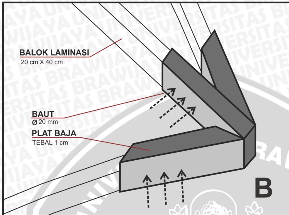
lampiran 45 Detail Sambungan B Bangunan Workshop
