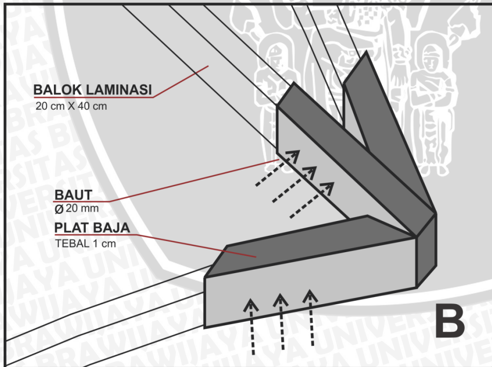
Lampiran 37 Detail Sambungan B Ruang Penerima
