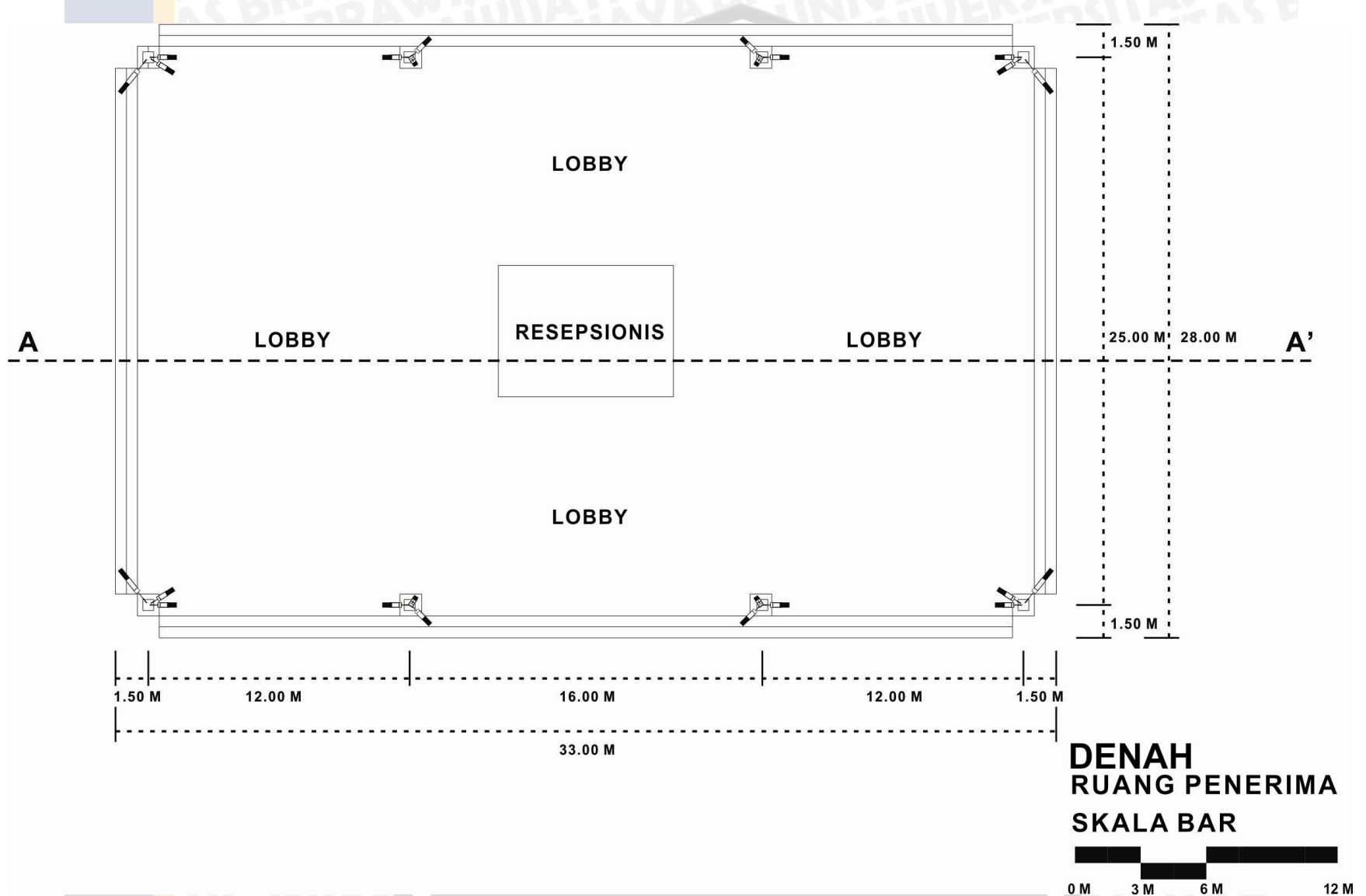
Lampiran 33 Denah Ruang penerima
