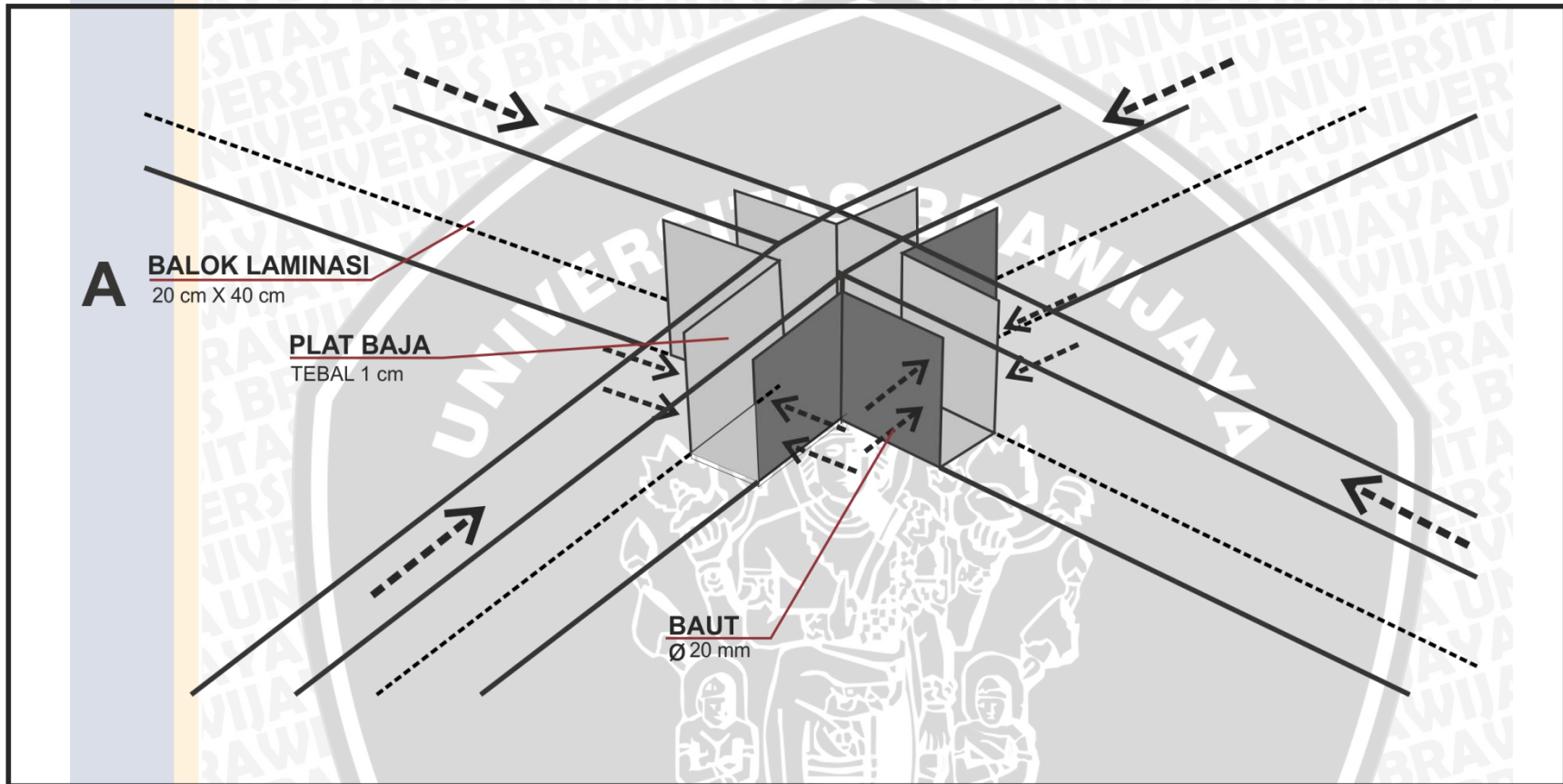
Lampiran 44 Detail Sambungan A Bangunan Workshop
