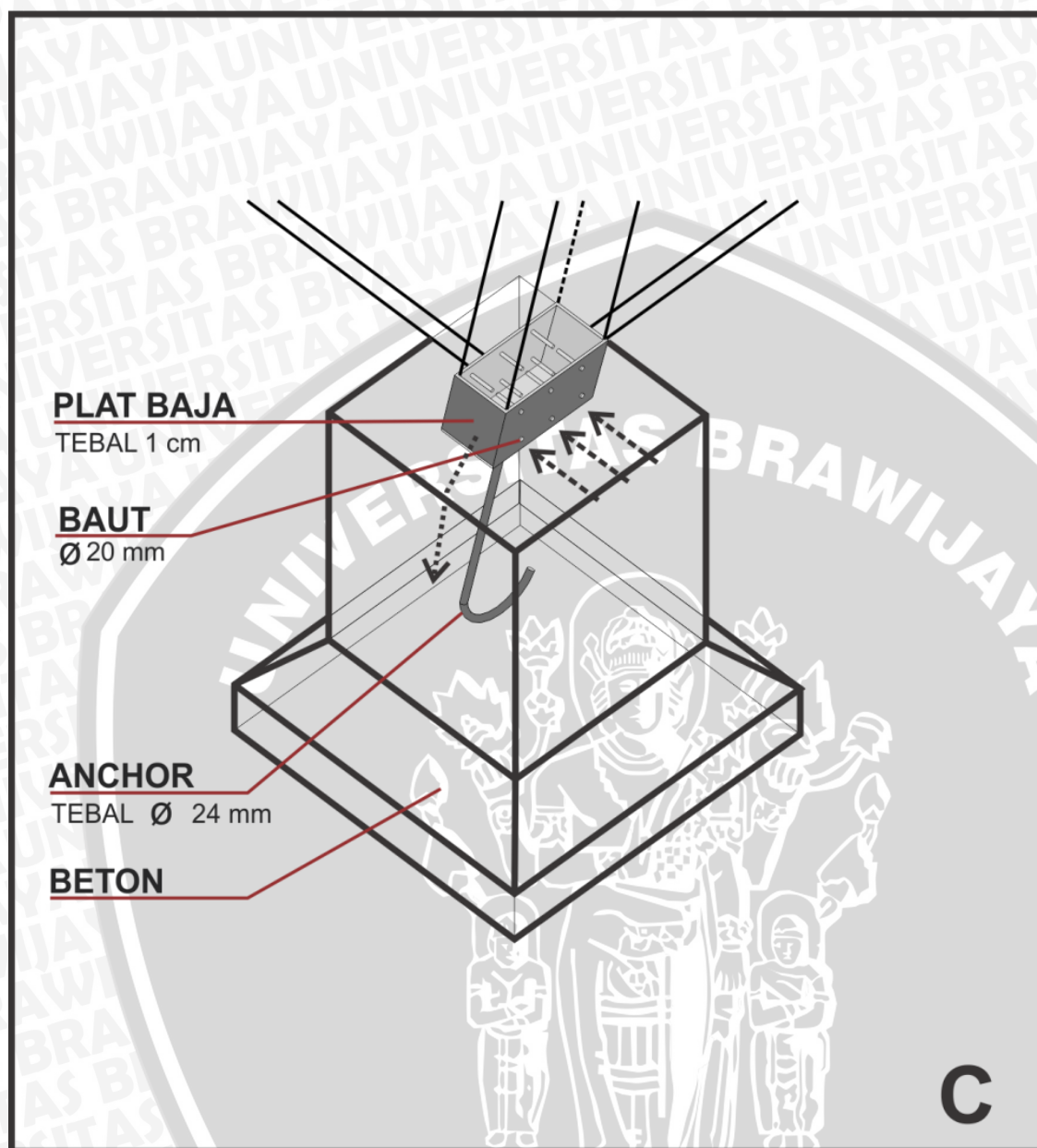
Lampiran 26 Detail C bangunan galeir
