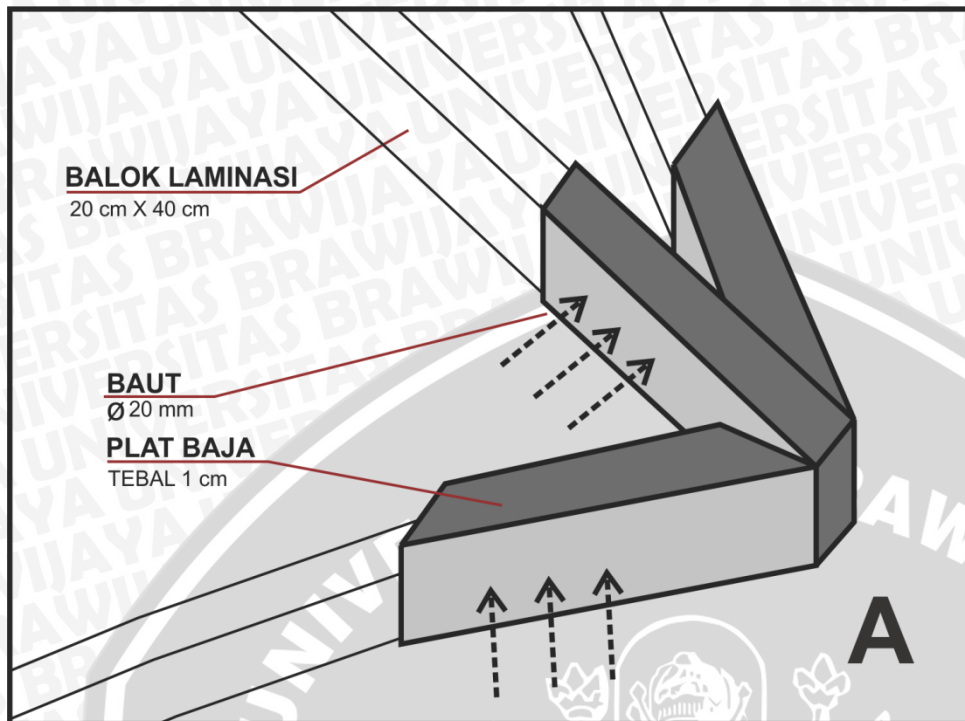
Lampiran 30 Detail Sambungan A Rest Area
