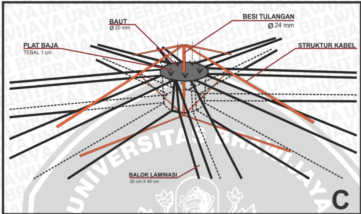
Lampiran 38 Detail Sambungan C Ruang penerima
