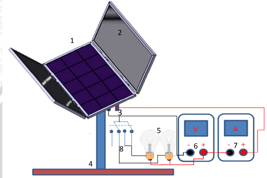
Gambar 3.7 Instalasi penelitian
