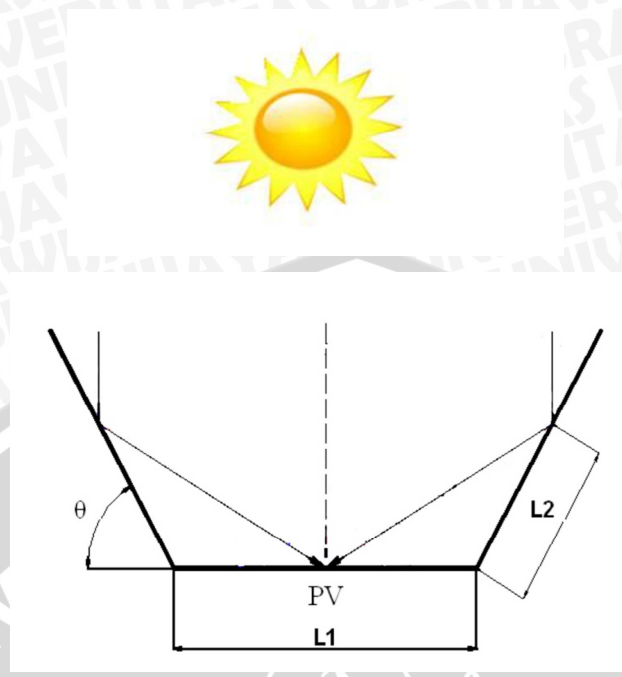
Gambar 3.1 Photovoltaic Mirror System
