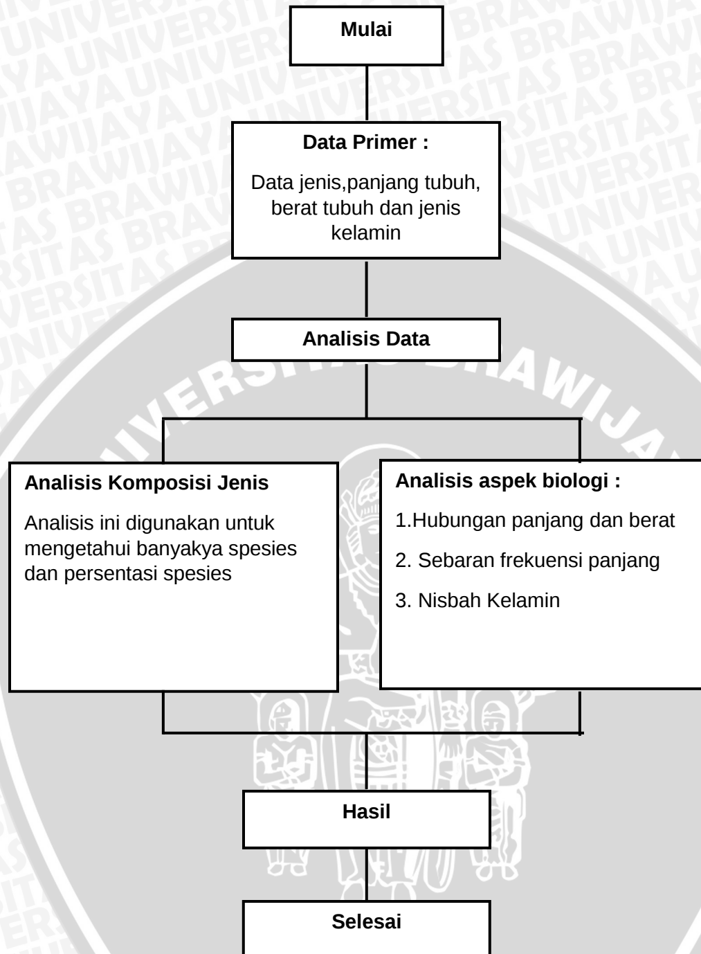
Gambar 4. Diagram Alur Penelitian
