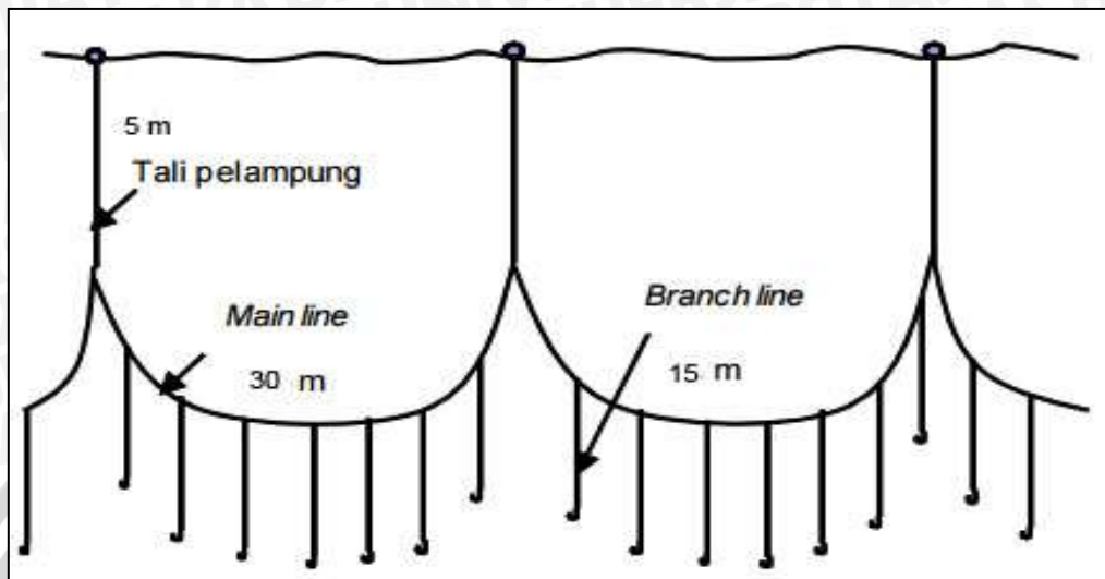
Alat Tangkap Pancing Rawai Cucut
