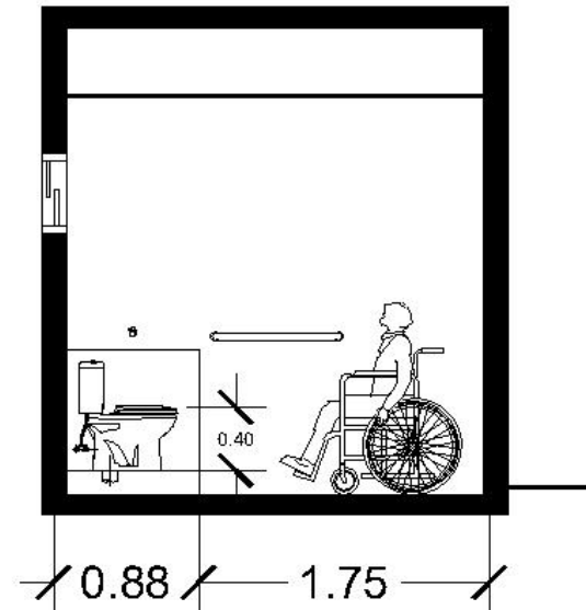
POT. KAMAR MANDI A
