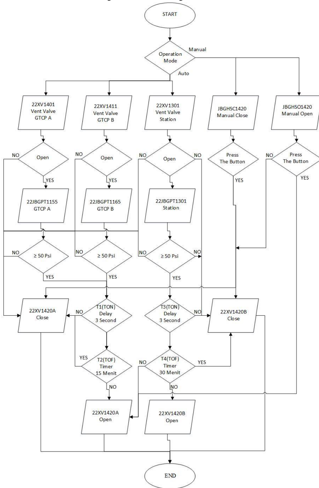
Lampiran 1 : Flowchat Sistem Pengaman N2 Snuffing Unit
